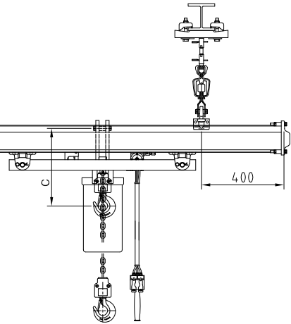
Double-girder crane
