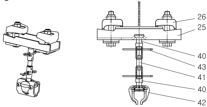
Suspension fitting
