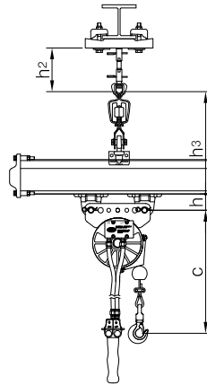
Single-girder crane
